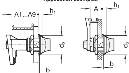
Cam door latches GN 119
