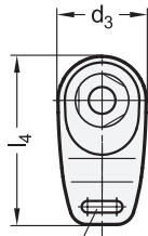
Slotted hole for key ring (ball chain)
